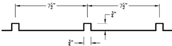
Figure 1. Spiral Rib Pipe Profile
