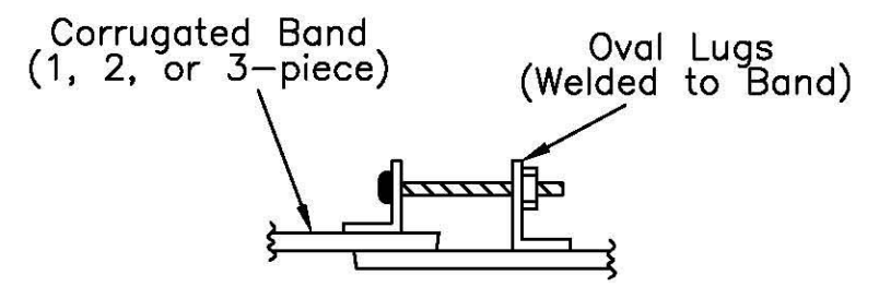
Detail "A"
