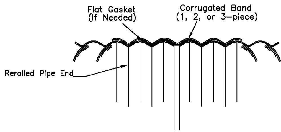
SECTION VIEW
