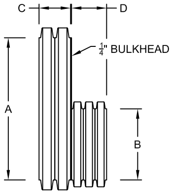
ELEVATION VIEW
