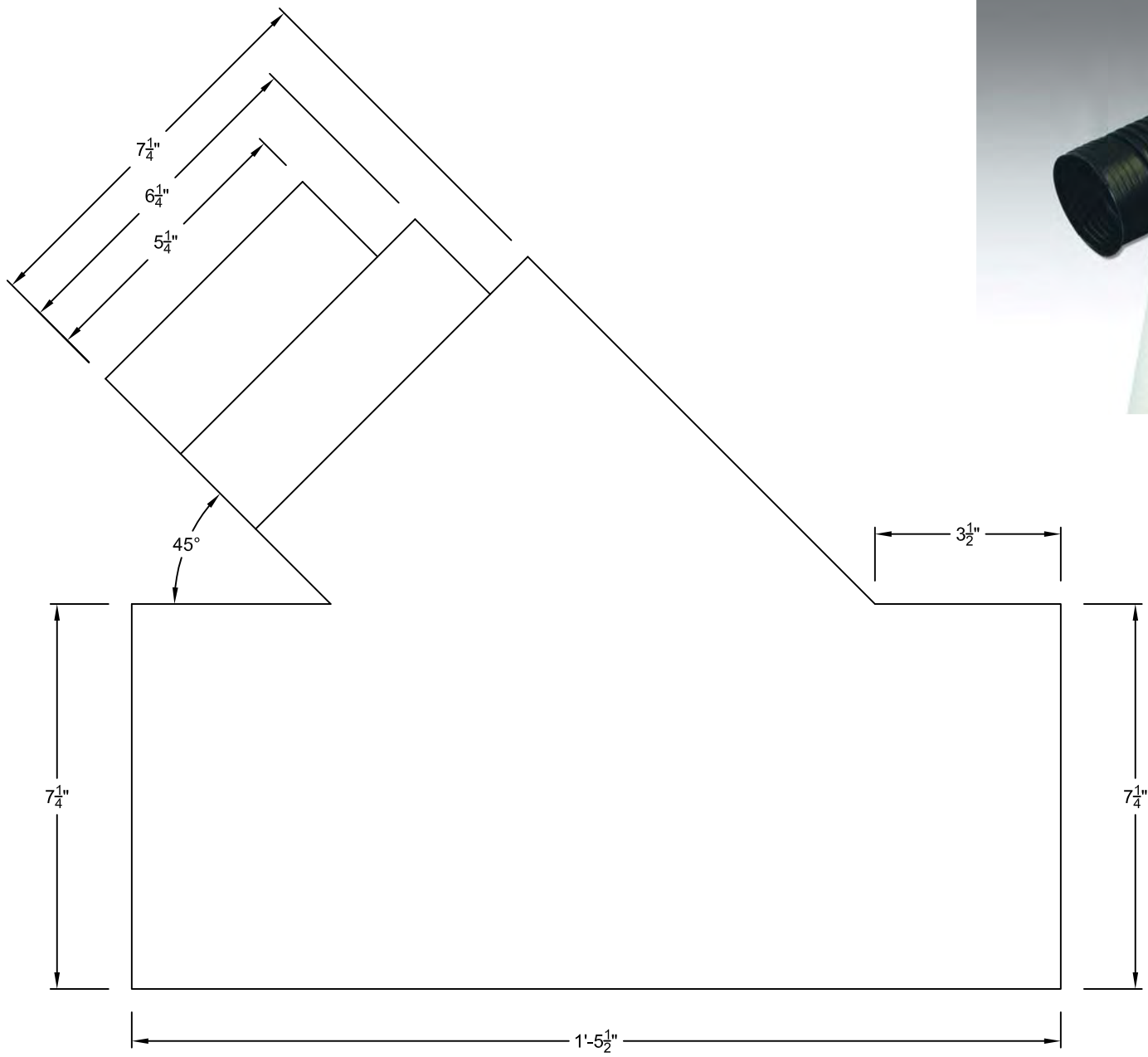
SIDE VIEW
