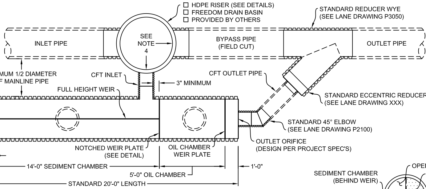
PLAN SECTION VIEW
